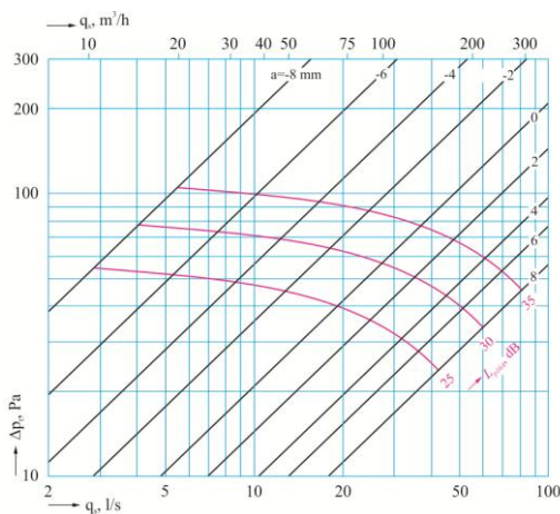
DVS-PY 125 mm
